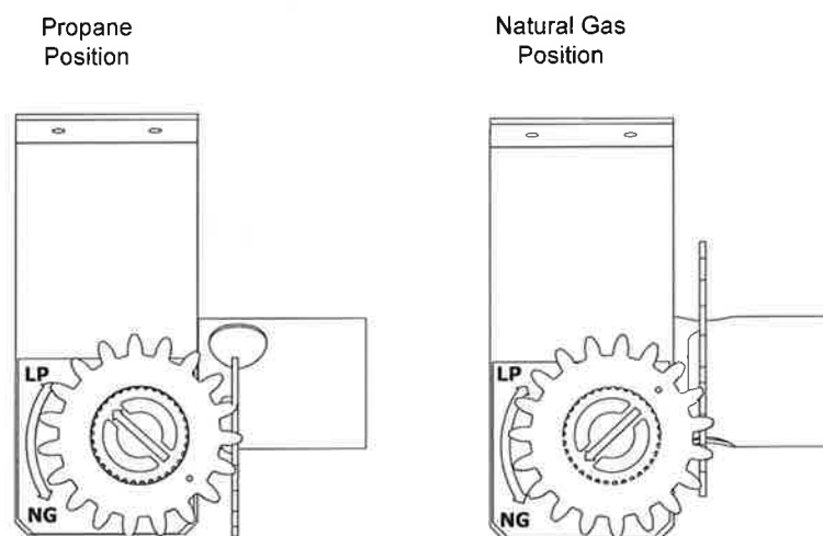
Fig. 8 - Selector Valve
