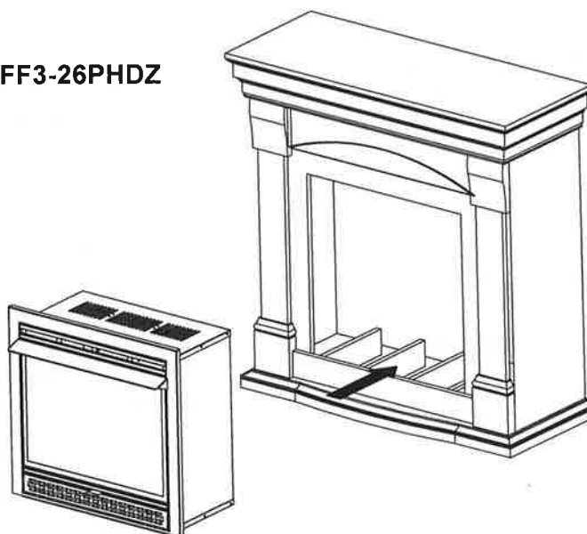
Fig. 2 - Insert Firebox
