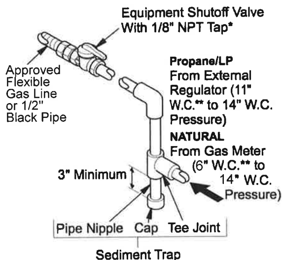
Fig. 10 - Gas Connection
