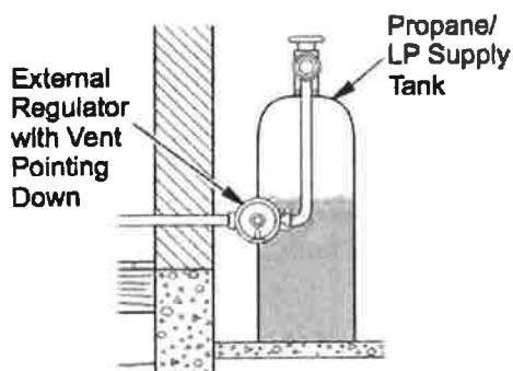
Fig. 9 - Regulator Conversion
