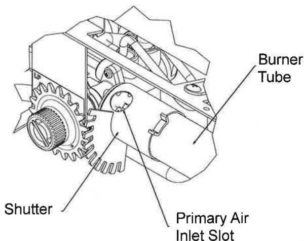
Fig. 24 - Primary Air Inlet Slot on Burner Tube
