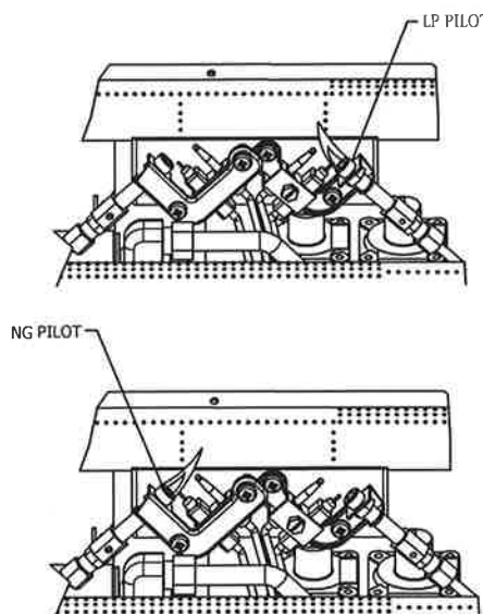
Fig. 21 - Incorrect Pilot Flame Pattern
