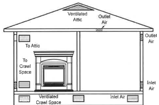
Fig. 5 - Ventilation Air from Outdoors
